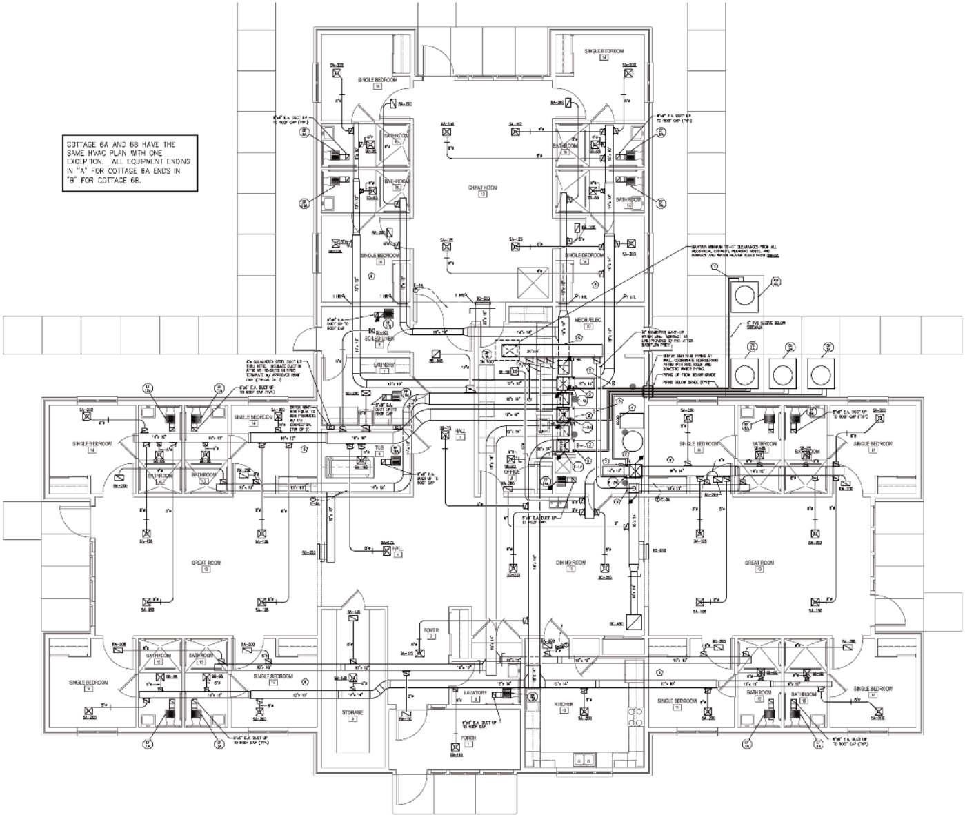
COTTAGE 6A FLOOR PLAN - HVAC SCALE: 1/4" = 1'-0"
